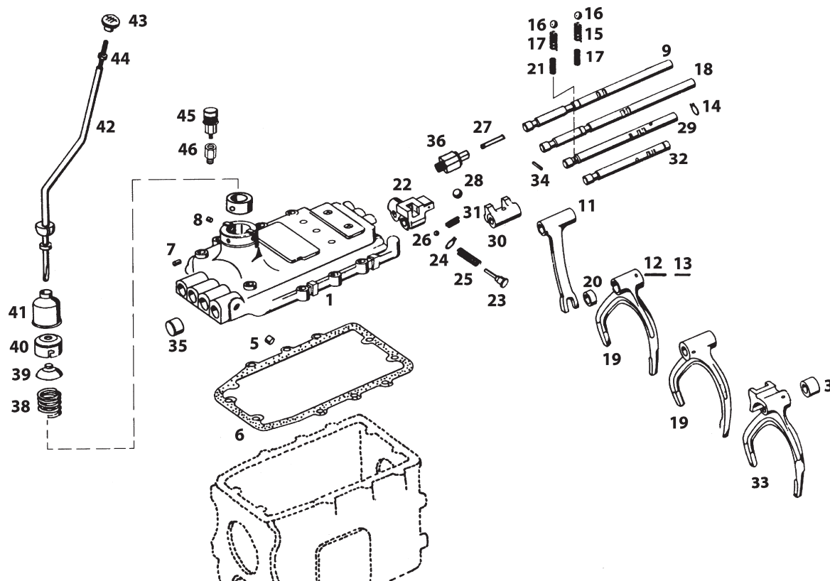
GEAR BOX (TOP COVER)
